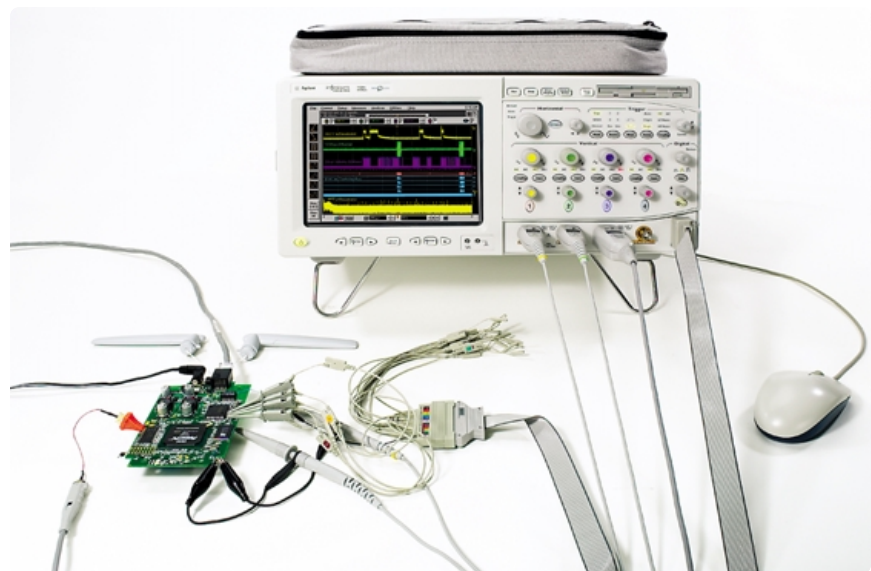
Figure 3. Using an Infiniium 54832D MSO to probe the analog and digital signals of a wireless LAN access point.
