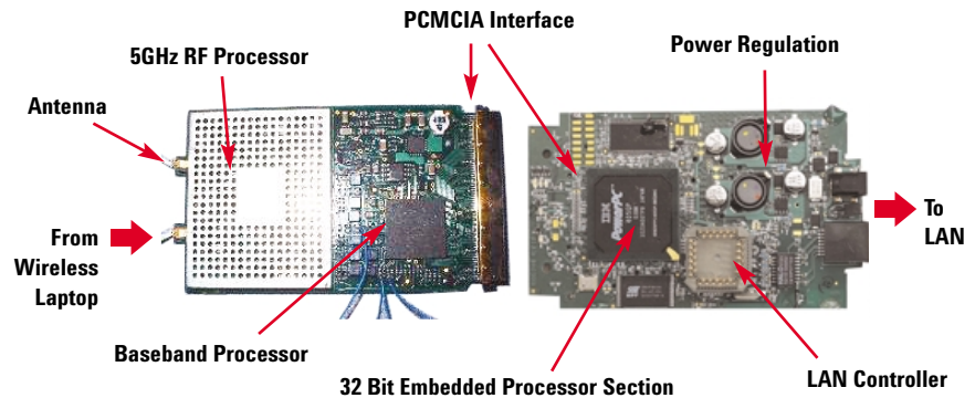
Figure 2. 802.11a 54-Mbps access point with boards unfolded.
