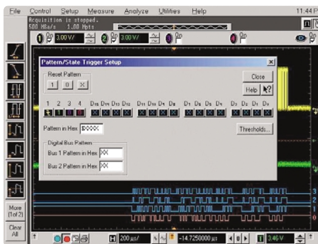
Figure 6. Triggering extends across all 20 channels with easy-to-use dialogs for quick trigger setups. MSOs have two pods of eight digital channels each, with connectors that are compatible with Agilent 16700 Logic Analyzers.
