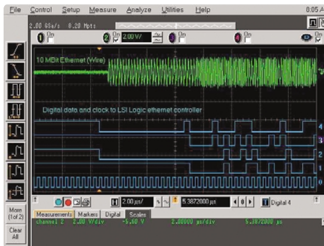
Figure 5. Use the MSO's 16 digital channels for triggering. The MSO is set to trigger on the 1010 pattern for a duration of 5 microseconds. With an ordinary four-channel DSO, the four channels would be used just to generate a trigger and there would be no channels left for debugging.
