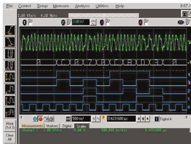
Figure 7. Digital signals can be grouped together by bus and viewed as hex value at every transition.
