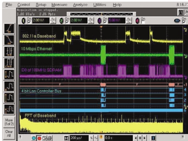
Figure 4. An MSO allows you to time correlate analog, digital, and spectral information all in one instrument.
