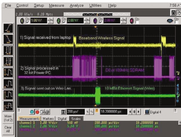
Figure 8. With an MSO, you can view a mix of signals. MegaZoom Deep memory lets you capture slow signals and then zoom in on the details fast without having to trigger twice.
